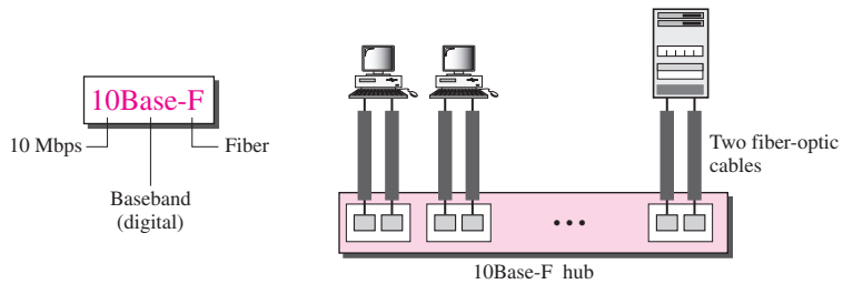
Figure 13.13 10Base-F implementation
