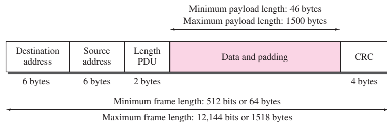
Figure 13.5 Minimum and maximum lengths
