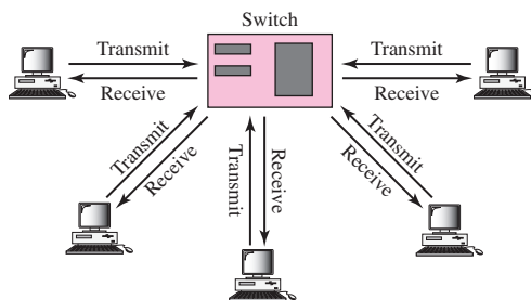
Figure 13.18 Full-duplex switched Ethernet
