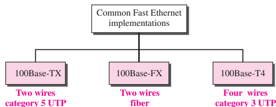
Figure 13.20 Fast Ethernet implementations
