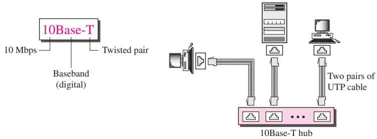
Figure 13.12 10Base-T implementation
