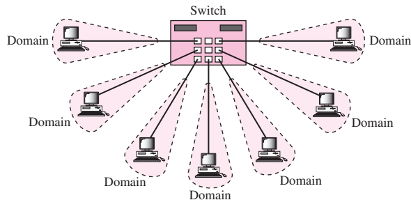
Figure 13.17 Switched Ethernet
