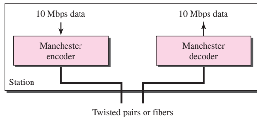
Figure 13.9 Encoding in a Standard Ethernet implementation
