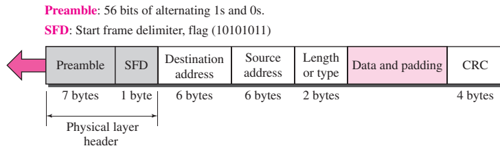
Figure 13.4 802.3 MAC frame
