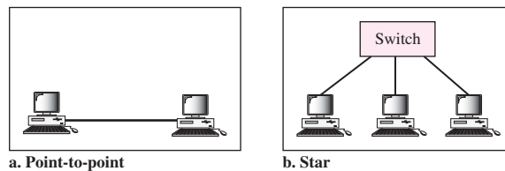
Figure 13.19 Fast Ethernet topology
