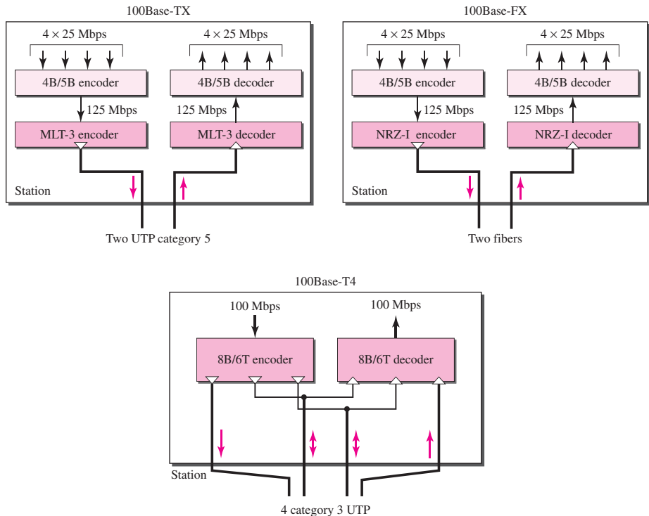
Figure 13.21 Encoding for Fast Ethernet implementation
