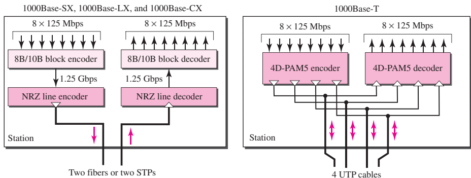
Figure 13.24 Encoding in Gigabit Ethernet implementations
