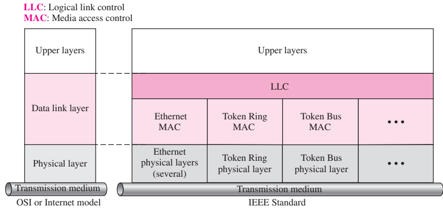
Figure 13.1 IEEE standard for LANs
