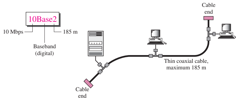
Figure 13.11 10Base2 implementation
