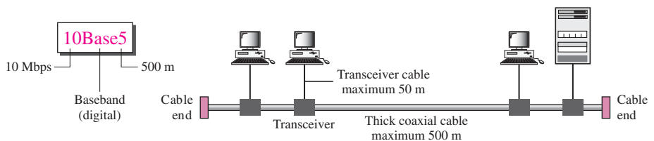
Figure 13.10 10Base5 implementation
