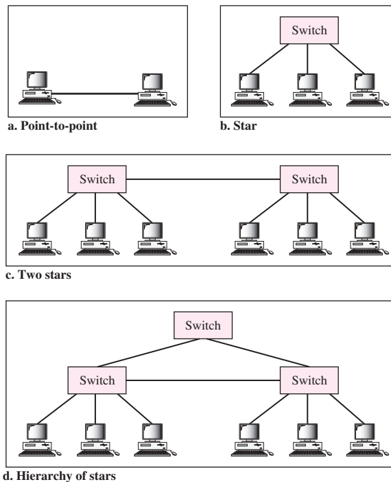
Figure 13.22 Topologies of Gigabit Ethernet
