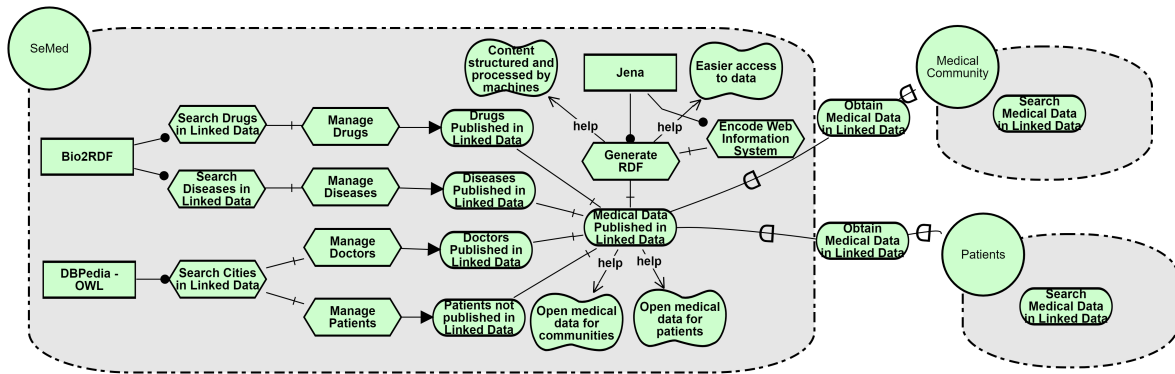
Figure 43 – iStar goal model for Semed.
