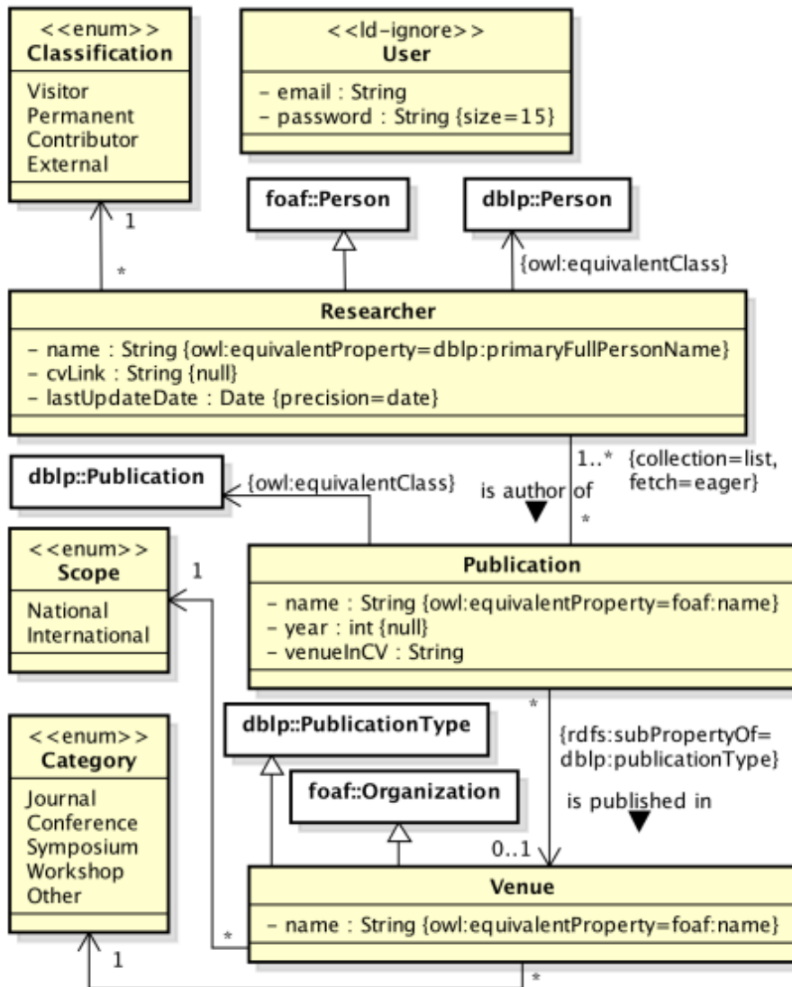
Figure 16 – A FrameWeb-LD Entity Model for C2D (CELINO et al., 2016).
