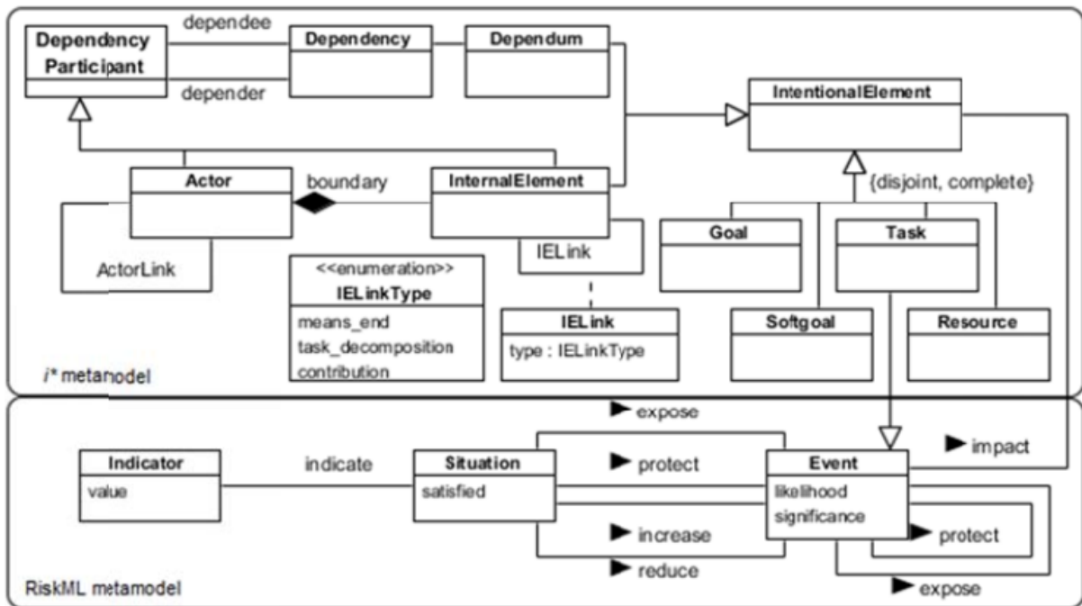
Figure 13 – RiskML-iStar Integrated Metamodel (COSTAL et al., 2015).
