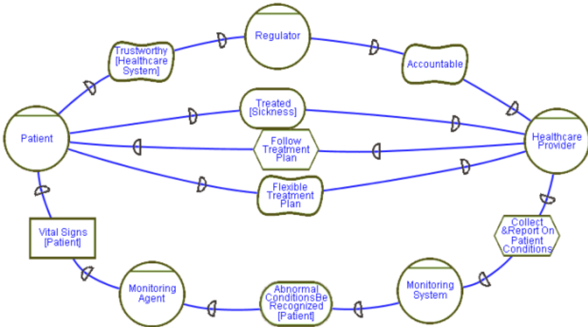
Figure 4 – A Strategic Dependency (SD) Model (YU, 2009).
