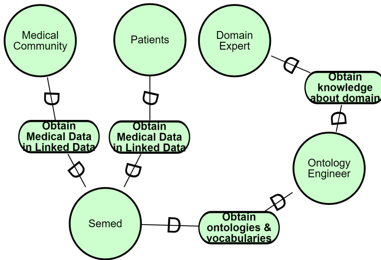
Figure 44 – iStar Semed goal model SD (Strategic Dependency) view.
