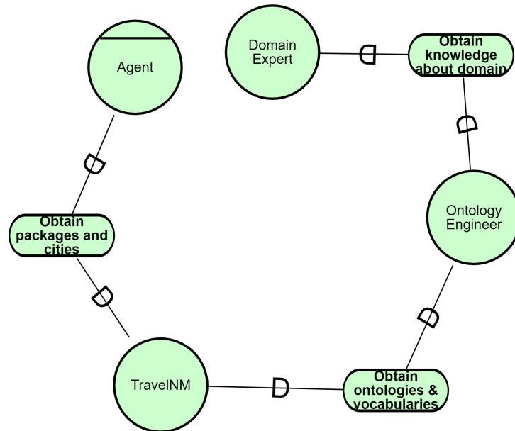
Figure 33 – iStar TravelNM goal model SD (Strategic Dependency) view.
