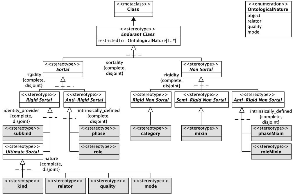
Figure 4: UML profile for OntoUML 2.
