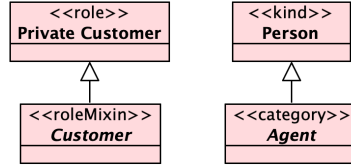
Figure 15: Counterexamples of nonSortalCantSpecializeSortal constraint.
