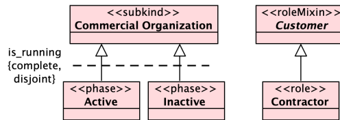
Figure 10: Counterexamples of sortalMustSpecializeUltimateSortal constraint.
