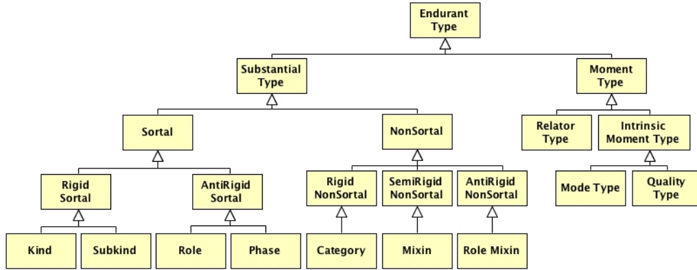
Figure 1: A Taxonomy of Endurant Types in UFO.
