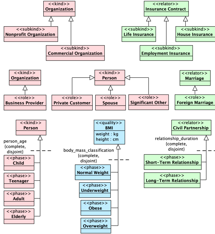
Figure 6: Examples of sortal classes represented in OntoUML.
