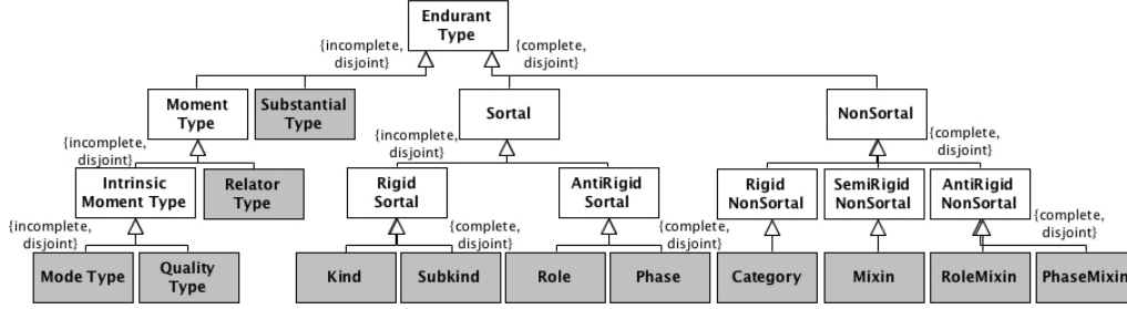
Figure 3: Proposed taxonomy of endurant types in UFO.
