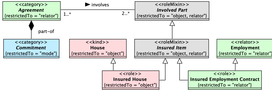
Figure 8: Examples of non-sortal classes with restrictedTo .
