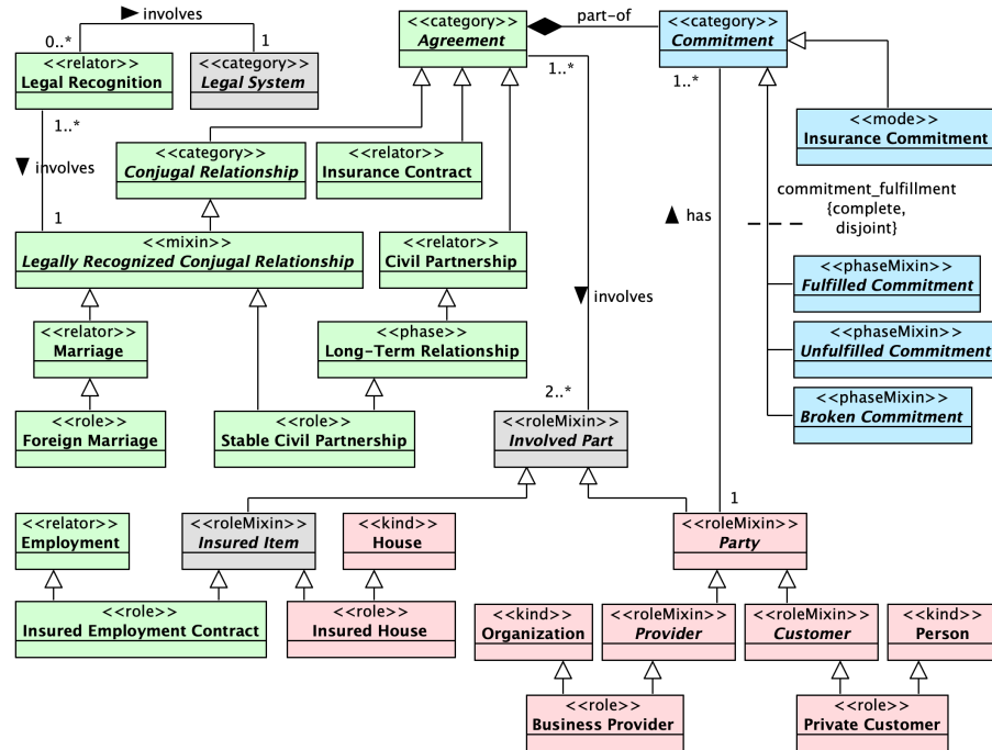
Figure 7: Examples of non-sortal classes.
