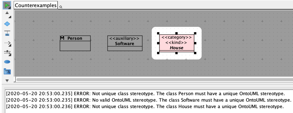
Figure 17: Screenshot of Visual Paradigm where the ontouml-vp-plugin presents to the modeler some verification issues.
