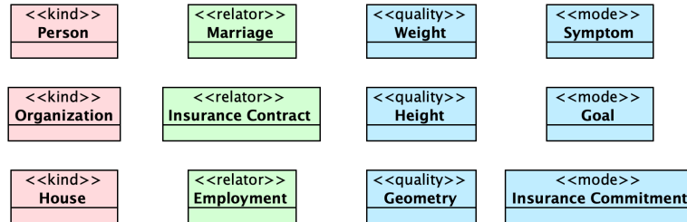
Figure 5: Examples of ultimate sortals represented in OntoUML.
