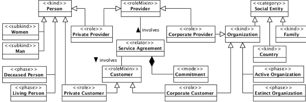
Figure 2: OntoUML example.
