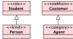
Figure 13: Counterexamples of rigidSortalCantSpecializeAntiRigid and rigidNonSortalCantSpecializeAntiRigid constraints.
