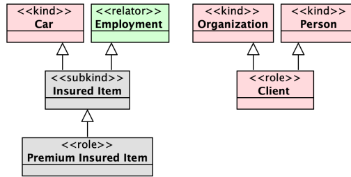
Figure 12: Counterexamples of cantSpecializeMoreThanOneUltimateSortal constraint.
