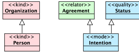
Figure 11: Counterexamples of ultimateSortalCantSpecializeAnother constraint.
