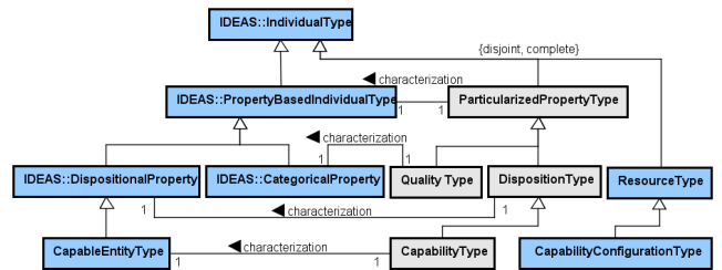
Figure 7. Fragment of the revised metamodel concerning Individual Types .
