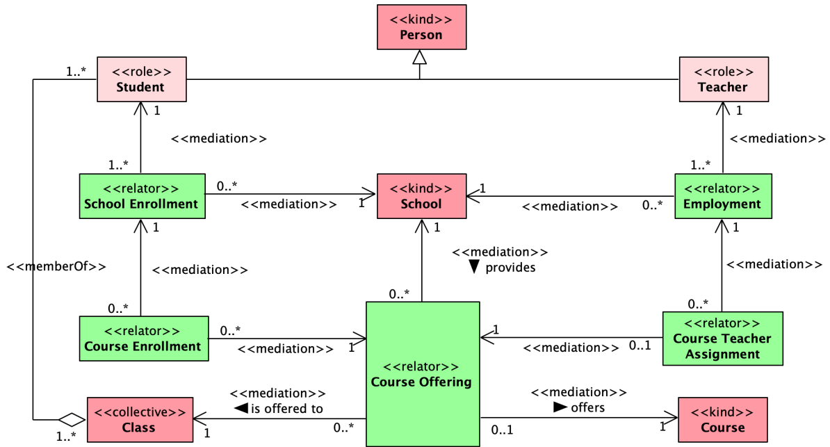
Figure 6. The School case in OntoUML.
