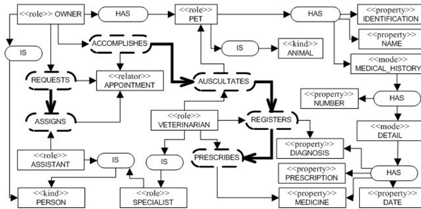
Fig. 3. Pre-conceptual schema of figure 1 after adding ontological labels to concepts.
