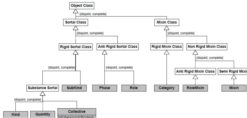
Fig. 2. Part of the proposed extension to UML diagrams for ontological purposes [8].
