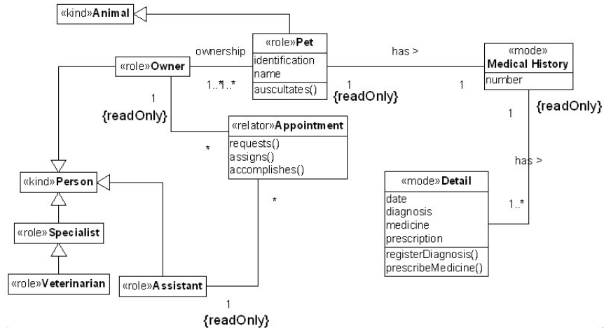
Fig. 4. Resulting class diagram from the pre-conceptual schema of figure 3.
