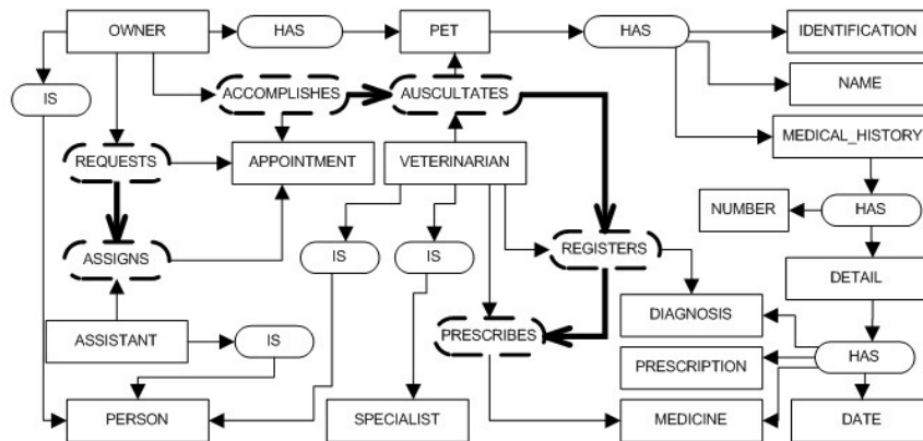
Fig. 1. An example of pre-conceptual schemas.
