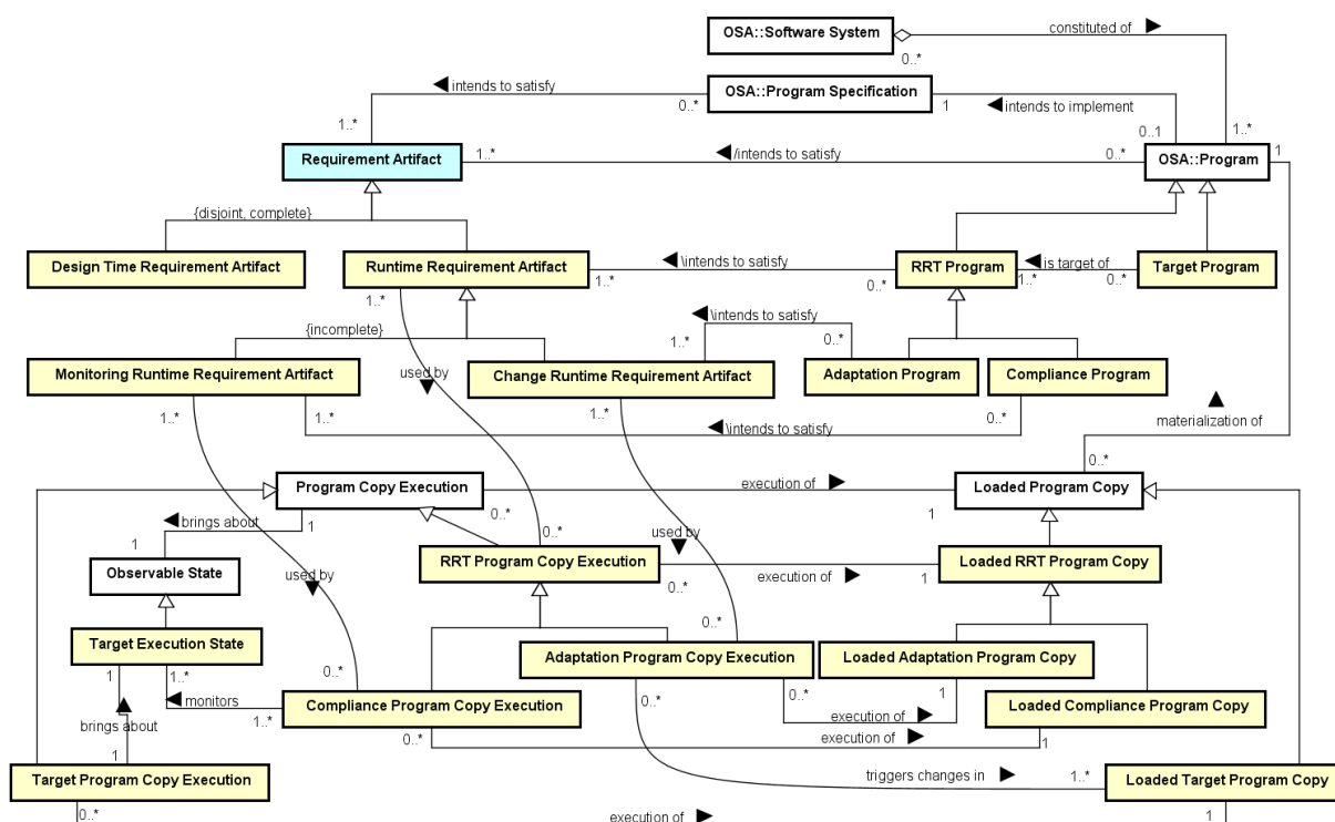
Fig. 15. Conceptual Model of RRO.
