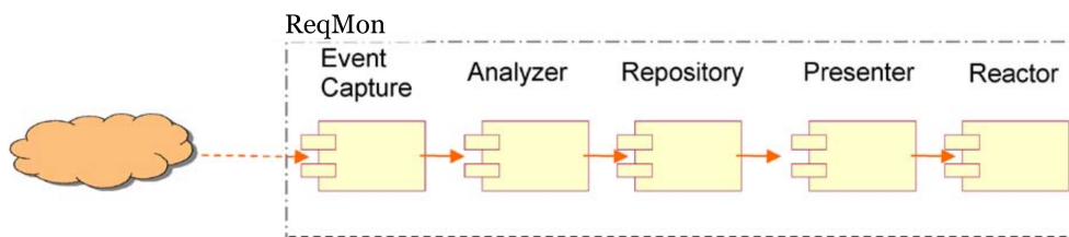
Fig. 4. ReqMon framework architecture (Robinson, 2006)
