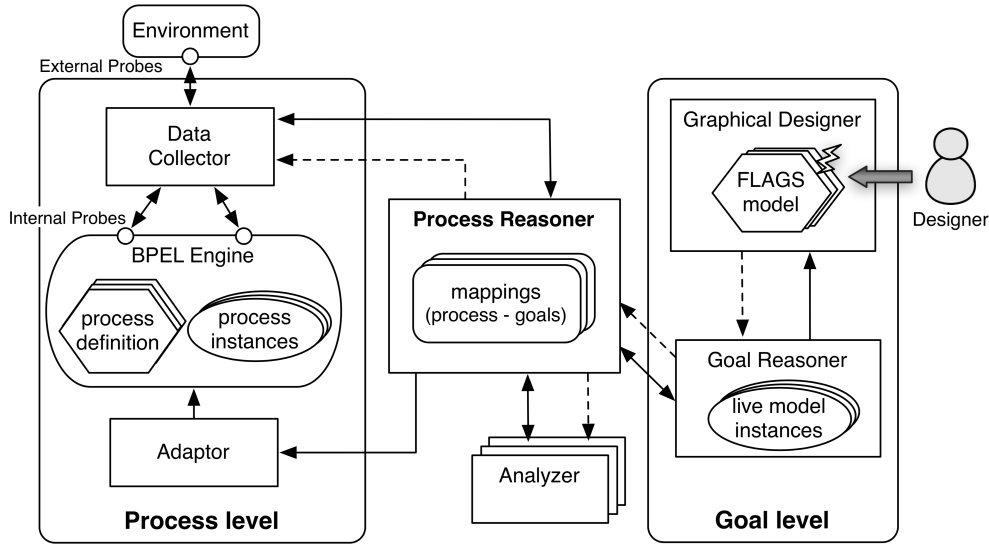
Fig. 6. FLAGS Runtime infrastructure (Pasquale et al., 2011)
