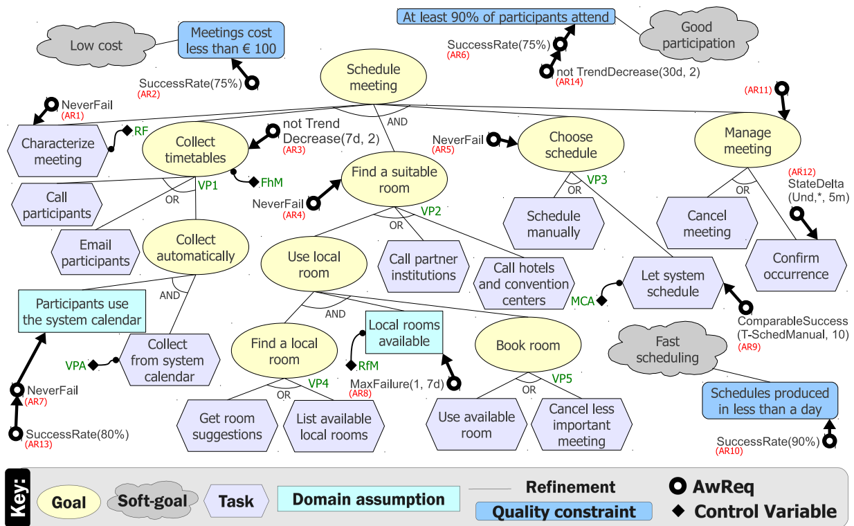
Fig. 3. Requirements model of a Meeting Scheduler, created with the Zanshin approach (Souza, 2012)
