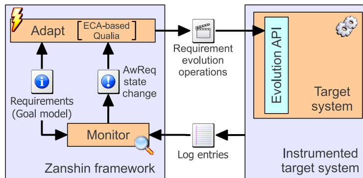
Fig. 2. Zanshin 's architecture representation (Souza, 2012)
