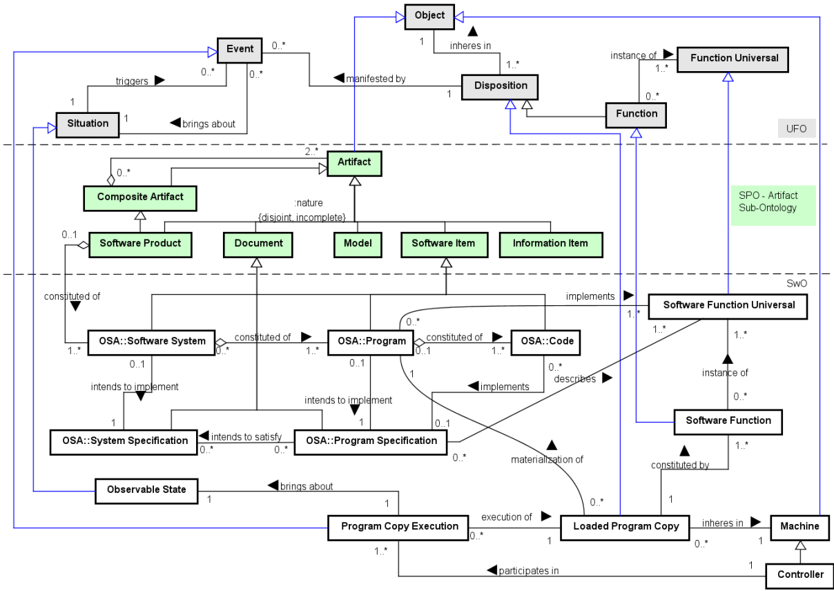
Fig. 13. Conceptual model fragment of SwO.
