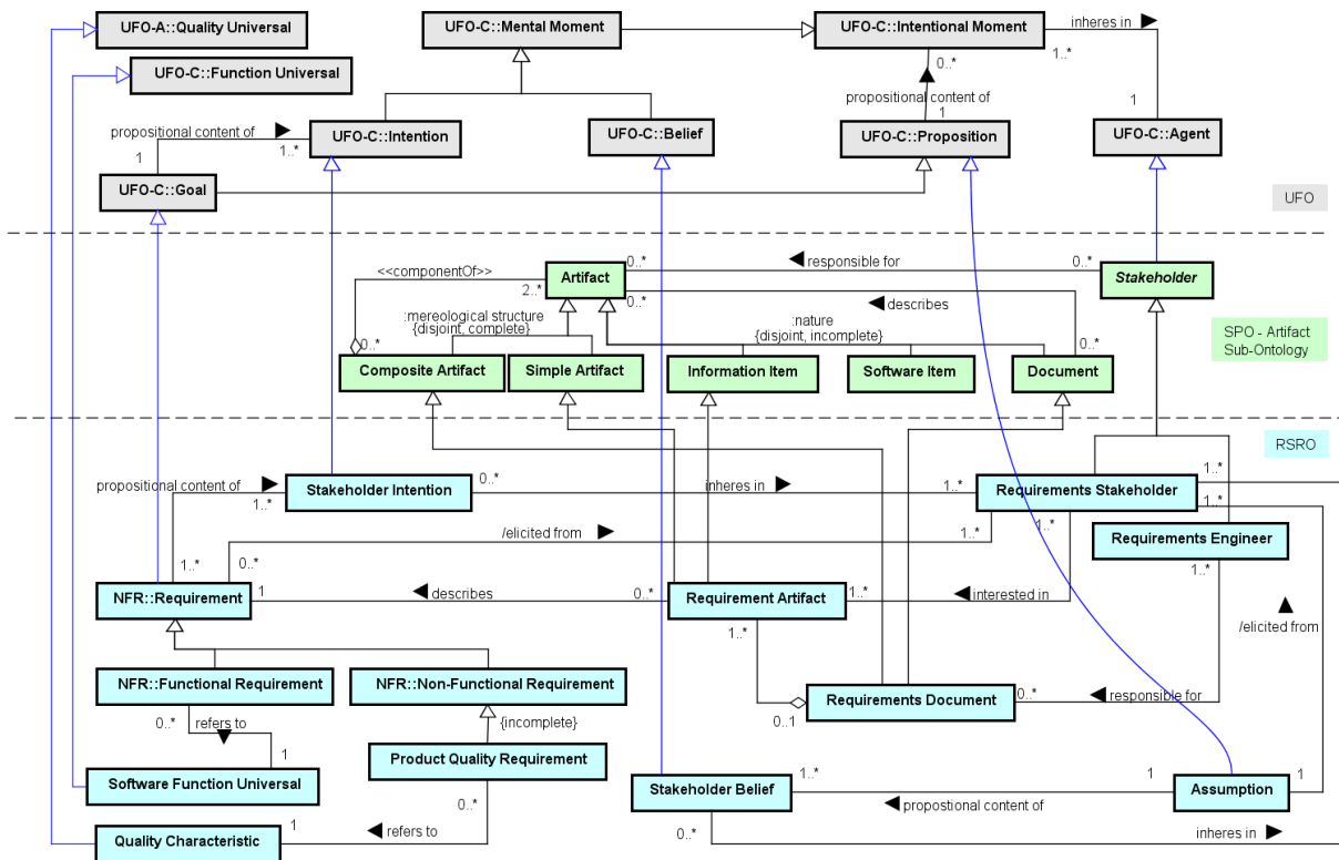
Fig. 14. Conceptual Model of RSRO.
