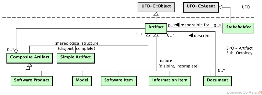
Fig. 12. SEON's view regarding Software and Related Artifacts.
