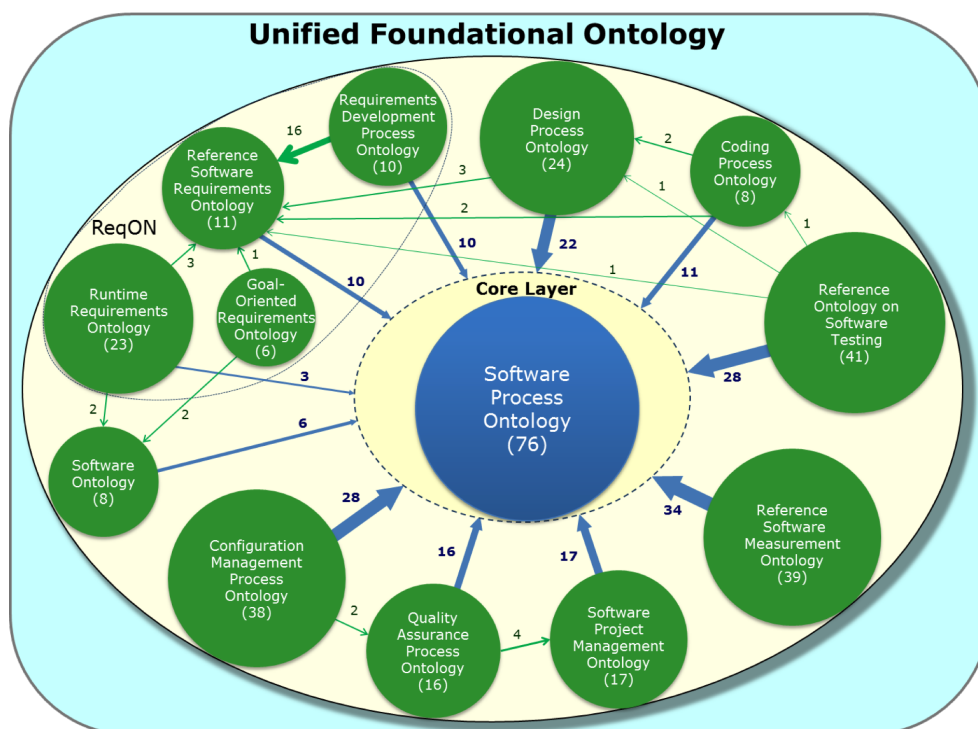
Fig. 11. SEON: The Network view (Ruy et al., 2016).
